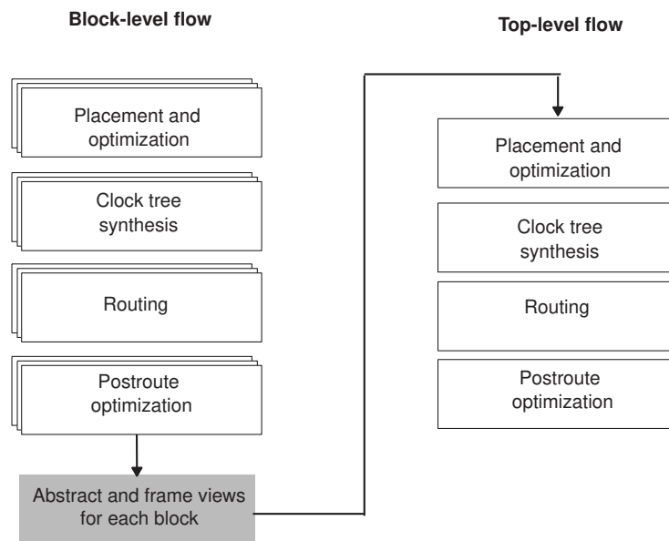
Figure 152 Top-Level Implemented After Blocks are Completed
