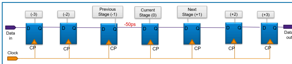
Figure 43 Previous, Current, and Next Path Stages
