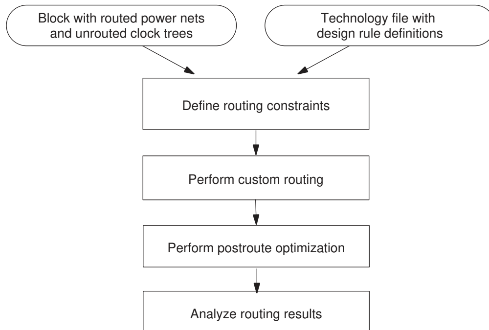
Figure 114 Basic Custom Router Flow
