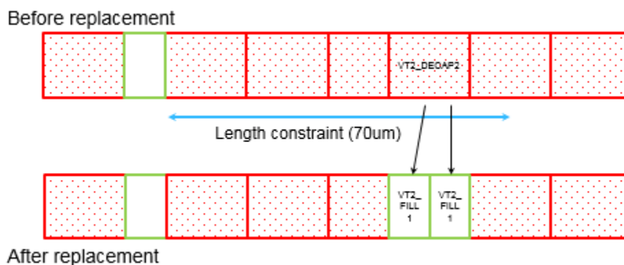
Figure 91 Fixing a Maximum Vertical Edge Length Violation
