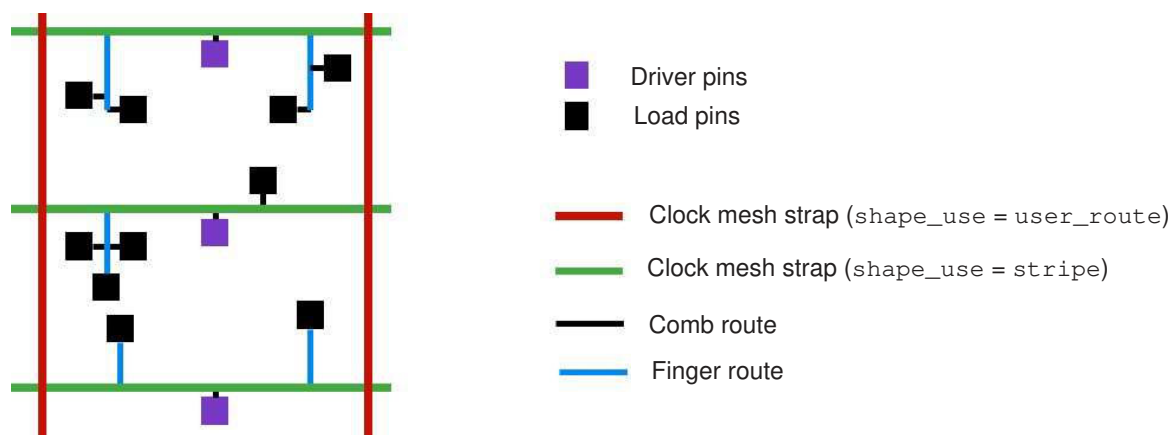
Figure 52 Fishbone Topology
