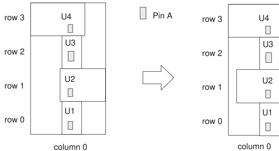
Figure 138 Minimizing the Column Width of a Relative Placement Group Aligned by Pins
