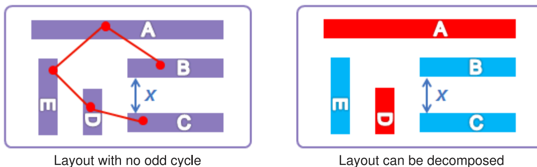
Figure 5 No Odd-Cycle Violation
