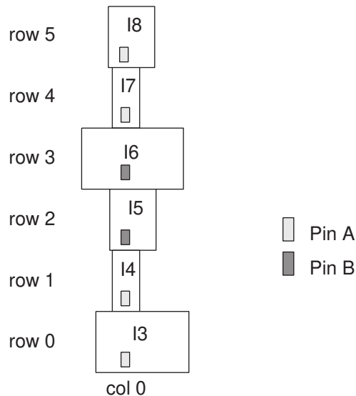
Figure 139 Relative Placement Group Aligned by Different Pins
