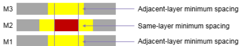
Figure 110 Minimum Spacing From Metal Fill to Critical Net Shape
