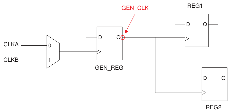
Figure 39 Generated Clock With Invalid Master Clock Source
