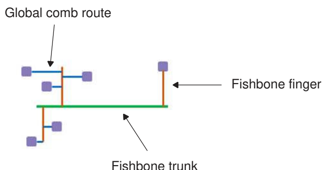
Figure 58 Detail Fishbone Routes and Global Comb Routes
