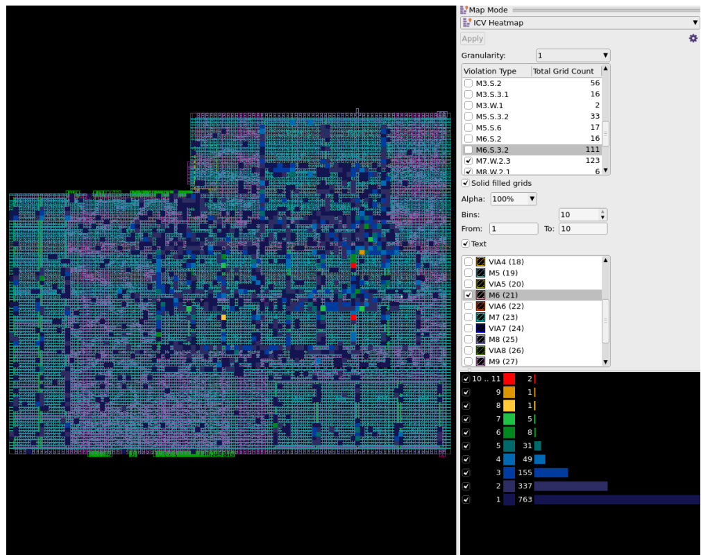
Figure 104 Selecting Layers in the ICV Heatmap
