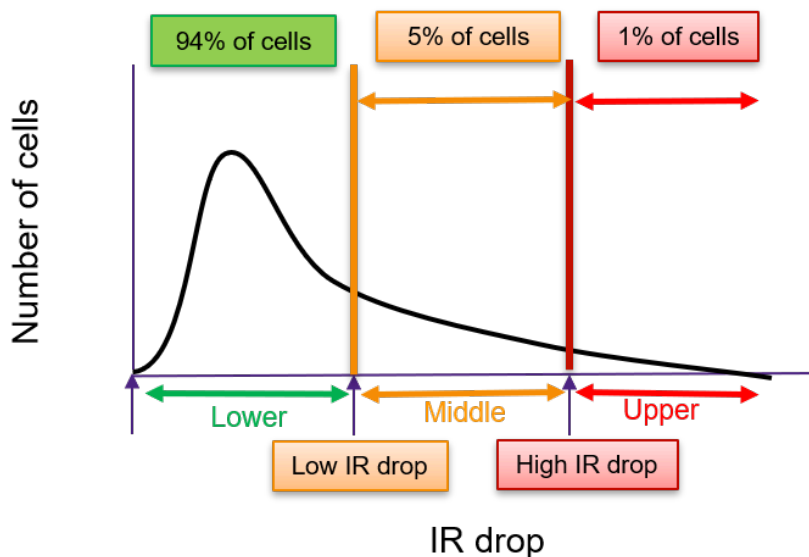
Figure 18 Default Cell Categories for IR-Drop-Aware Placement
