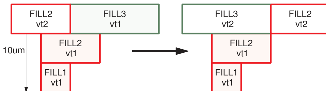
Figure 93 Fixing Maximum Stacking Violation by Reordering
