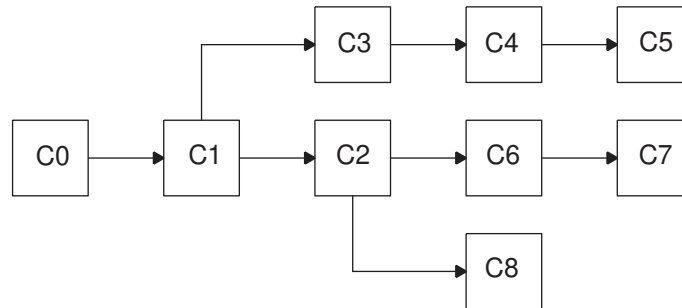
Figure 26 Example of Pulling Cells in a Contiguous Data Path
