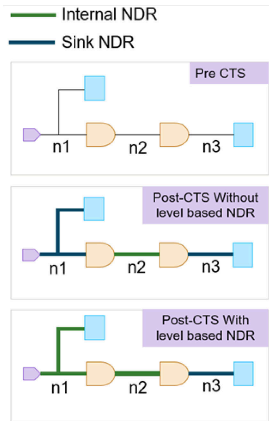
Figure 24 Level-Based Clock Nondefault Routing Rule
