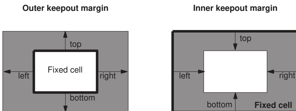
Figure 17 Placement Keepout Margins
