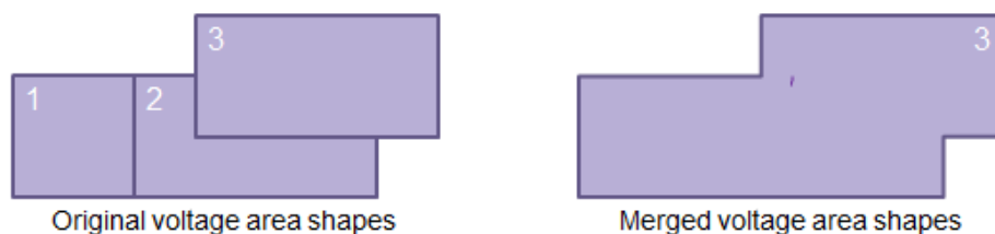
Figure 7 Merging Voltage Area Shapes
