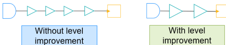
Figure 42 Improving the Repeater Levels in Clock Tree
