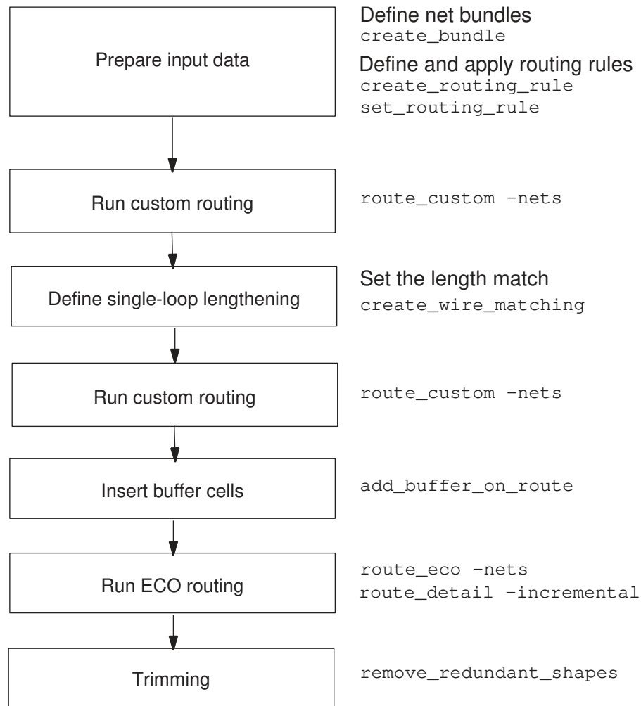
Figure 126 A Basic DDR Flow
