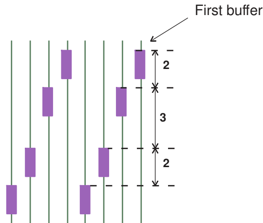
Figure 177 Buffer Patterns for a Vertical Bus
