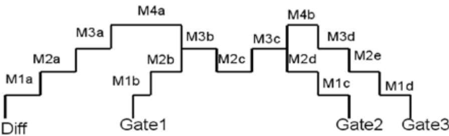
Figure 86 Layout Example for Antenna Recognition Modes
