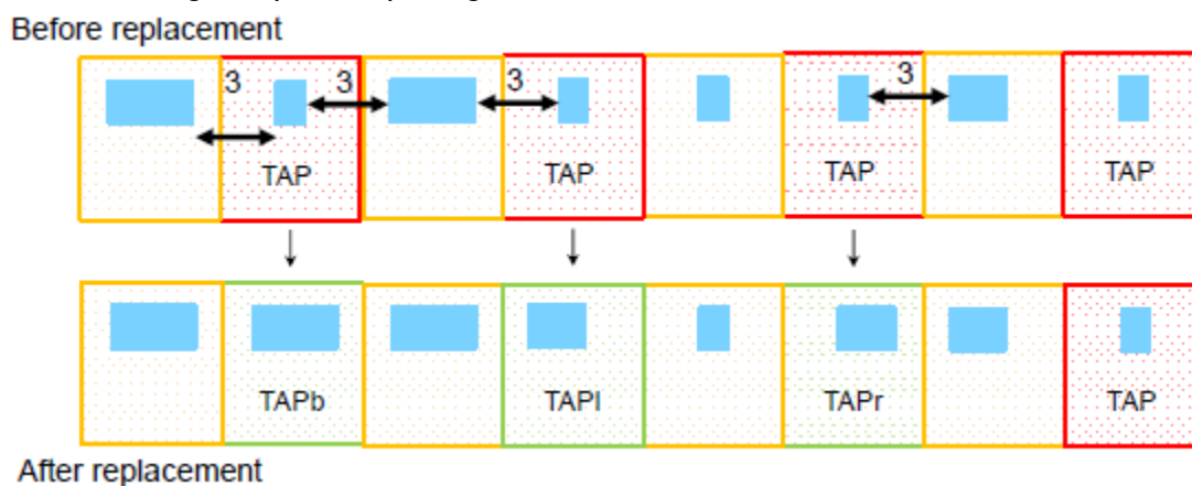
Figure 95 Fixing a Tap Cell Spacing Violation
