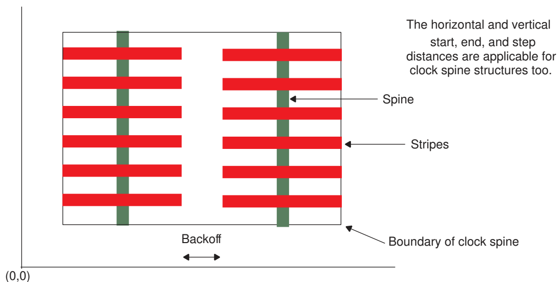
Figure 51 Clock Spine Structure
