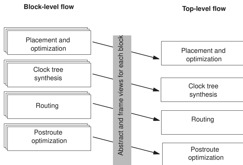
Figure 153 Top and Block Levels Implemented in Parallel
