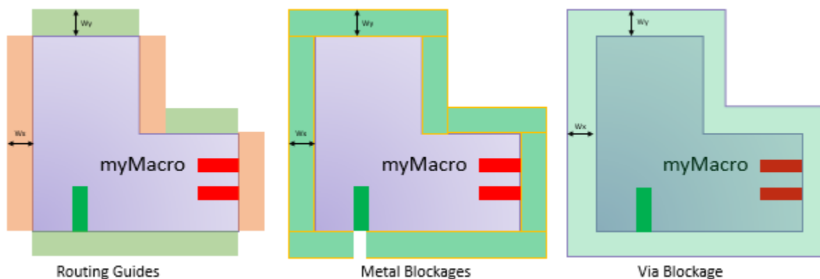
Figure 61 Pin Access Routing Guides and Blockages
