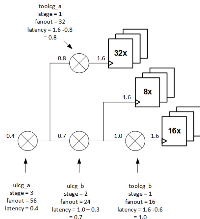
Figure 16 Latency Calculations With Varying Fanout
