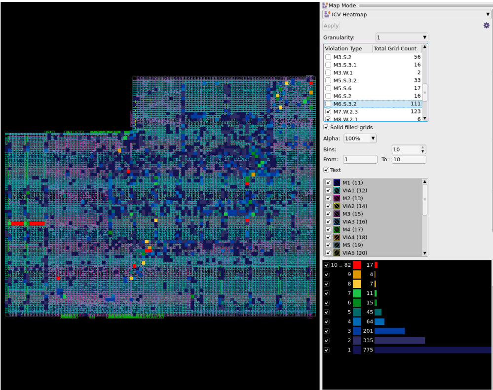
Figure 98 Violation Type in ICV Heat Map
