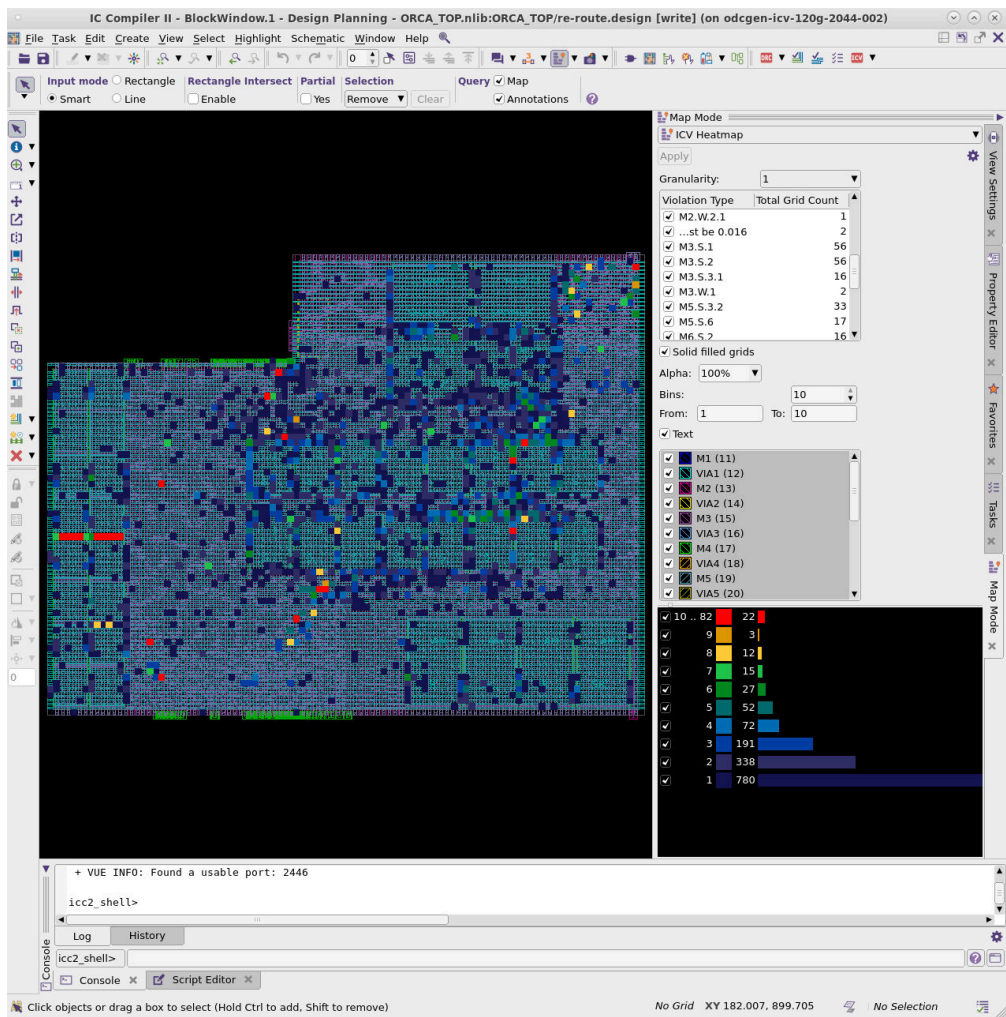
Figure 96 ICV Heat Map
