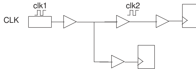
Figure 34 Cascaded Clock With Two Source Clocks
