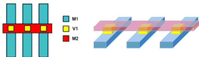
Figure 71 Single-Level Pattern-Based Must-Join Pin Connection
