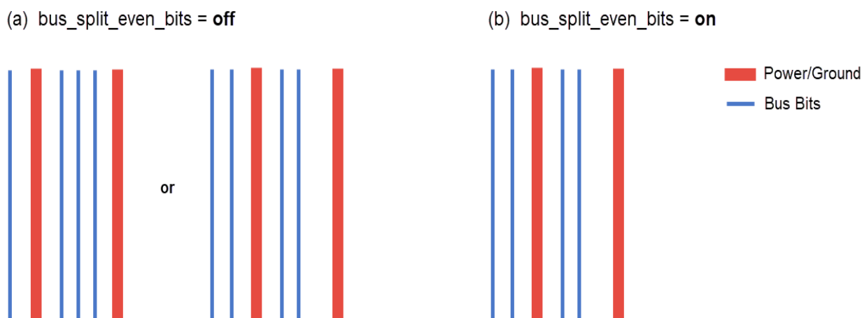
Figure 124 Splitting Bus Trunk to Route Through Power and Ground Rails
