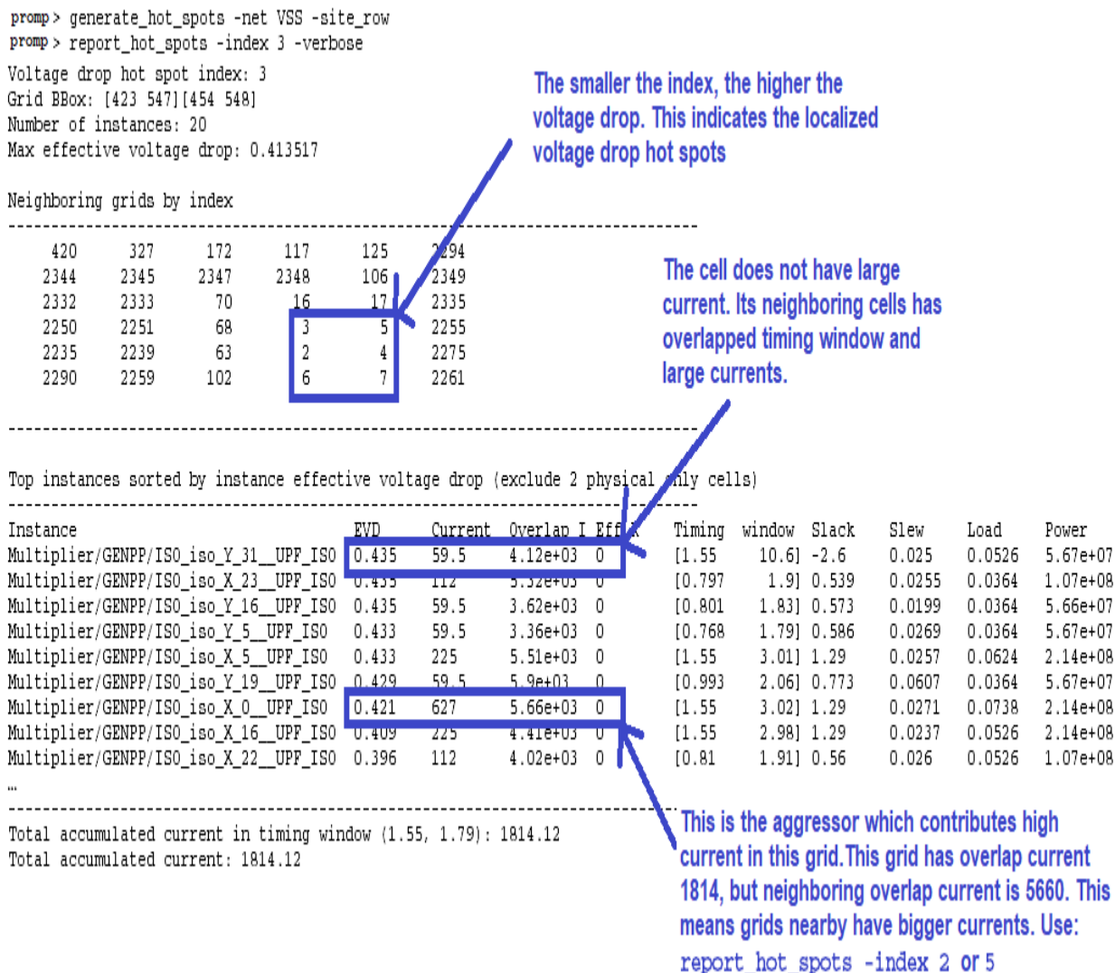
Figure 172 Checking High Voltage Drop Caused by Overlapping Timing Window (I)
