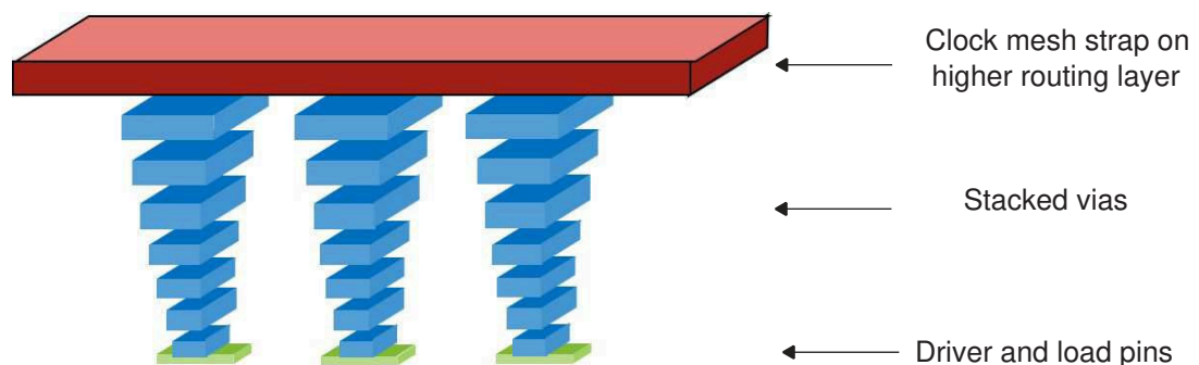
Figure 56 Vias in the Comb Topology
