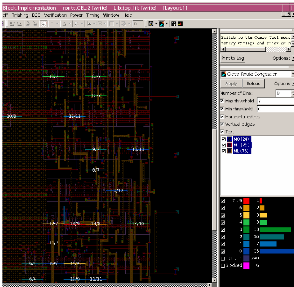
Figure 80 Global Route Overflow on Global Routing Cell
