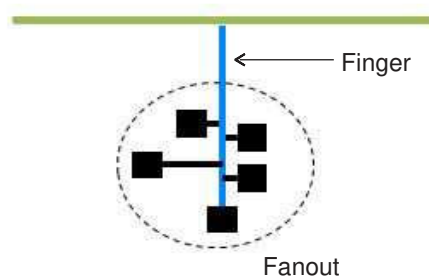
Figure 53 Fanout of a Finger of the Fishbone Topology
