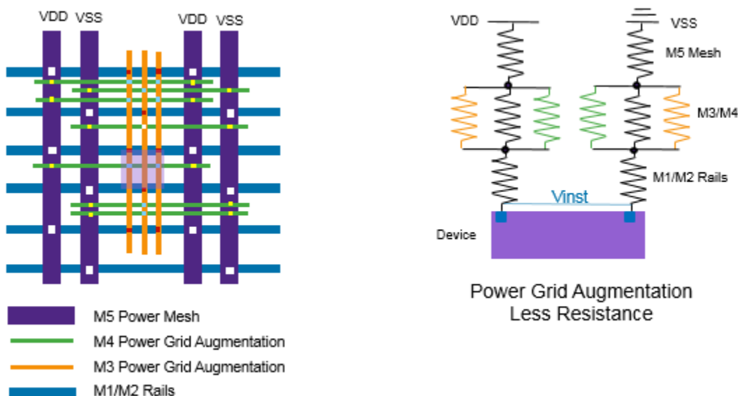
Figure 109 Power Grid Augmentation
