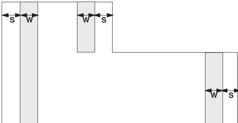
Figure 65 Routing Guide Perimeter Constraint Objects
