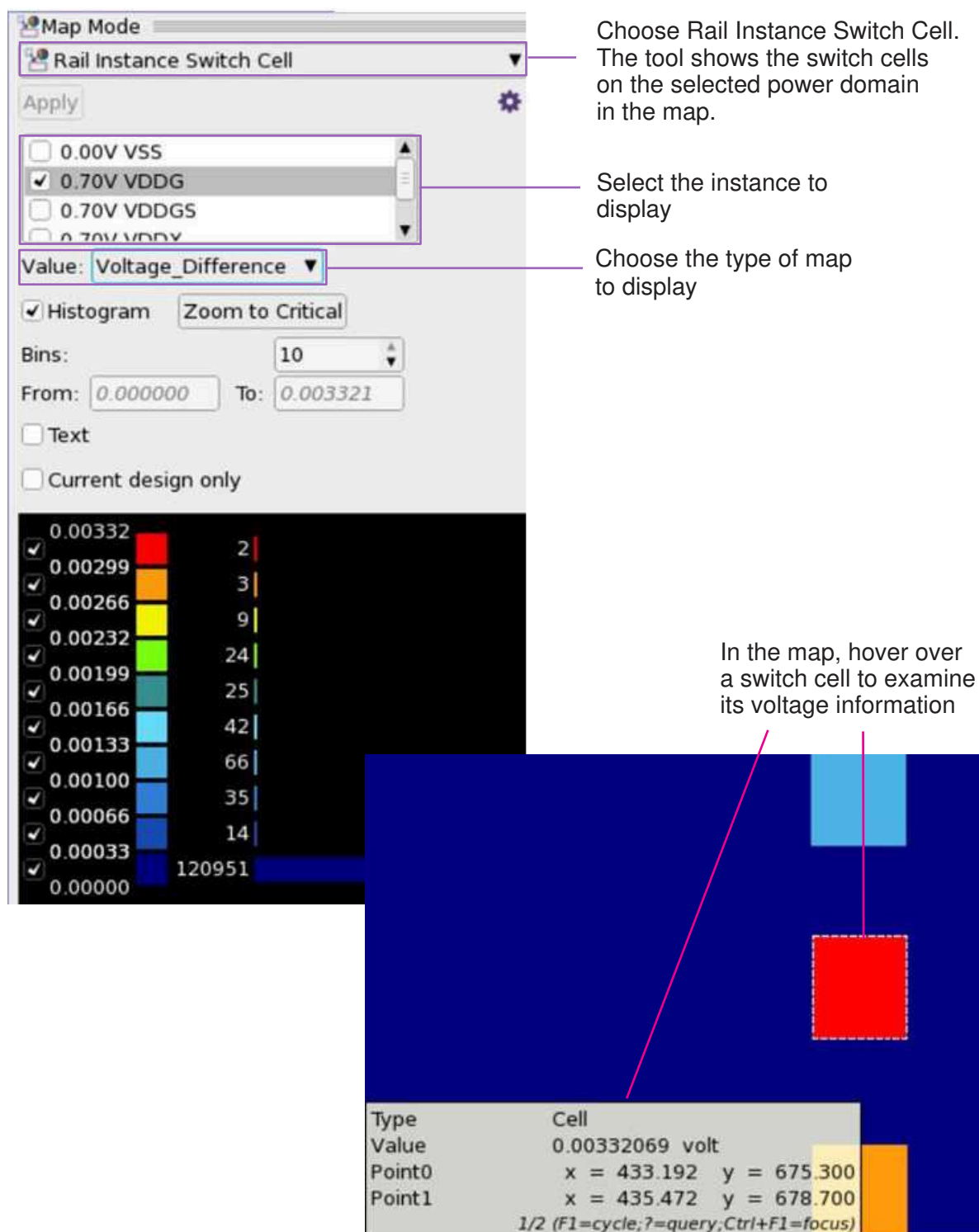
Figure 170 Displaying Maps for Switch Cells
