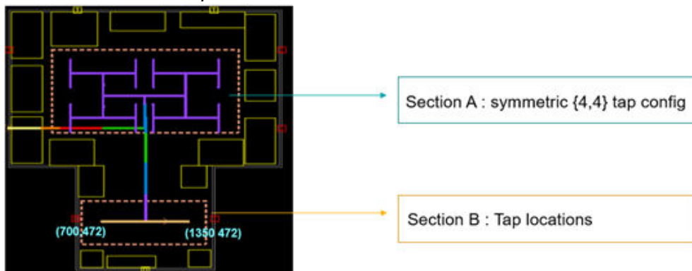
Figure 48 MSCTS Multiple H-Tree
