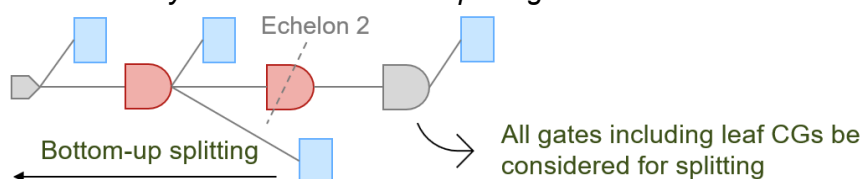
Figure 41 Latency Driven Clock-Gate Splitting
