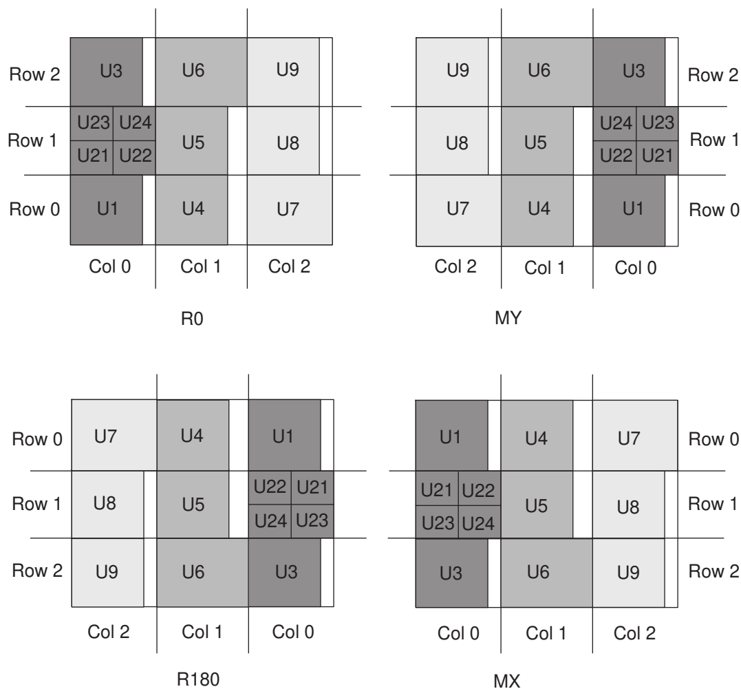
Figure 143 Orientation of Relative Placement Groups
