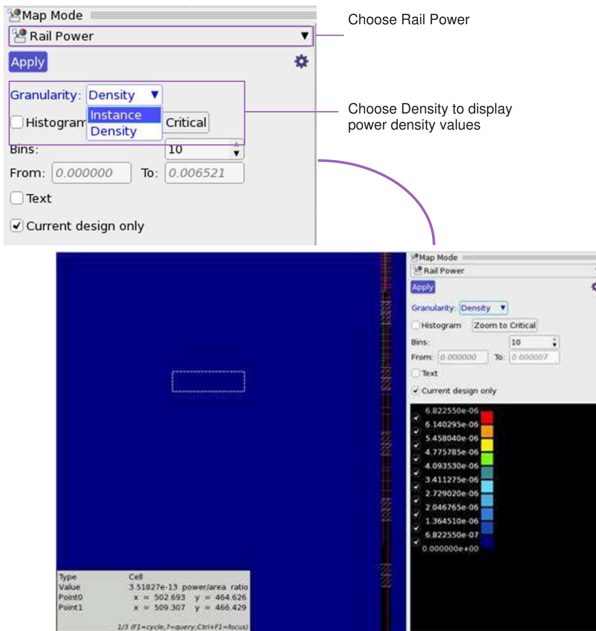
Figure 171 Displaying a Power Density Map
