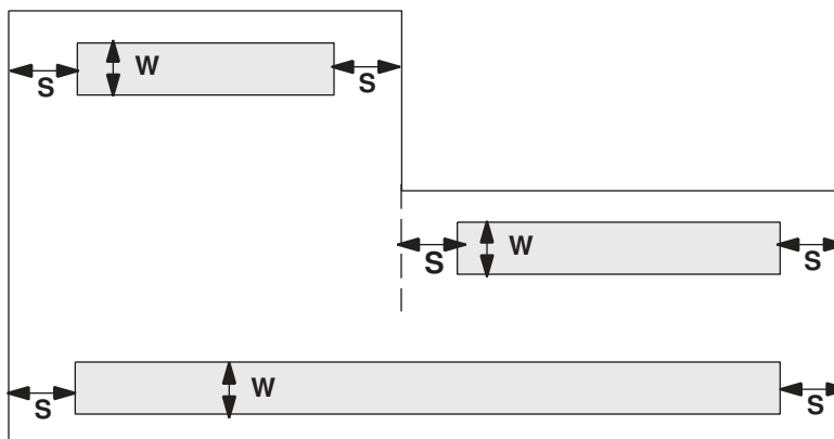
Figure 62 Continuous Metal Shape Perimeter Constraint Objects
