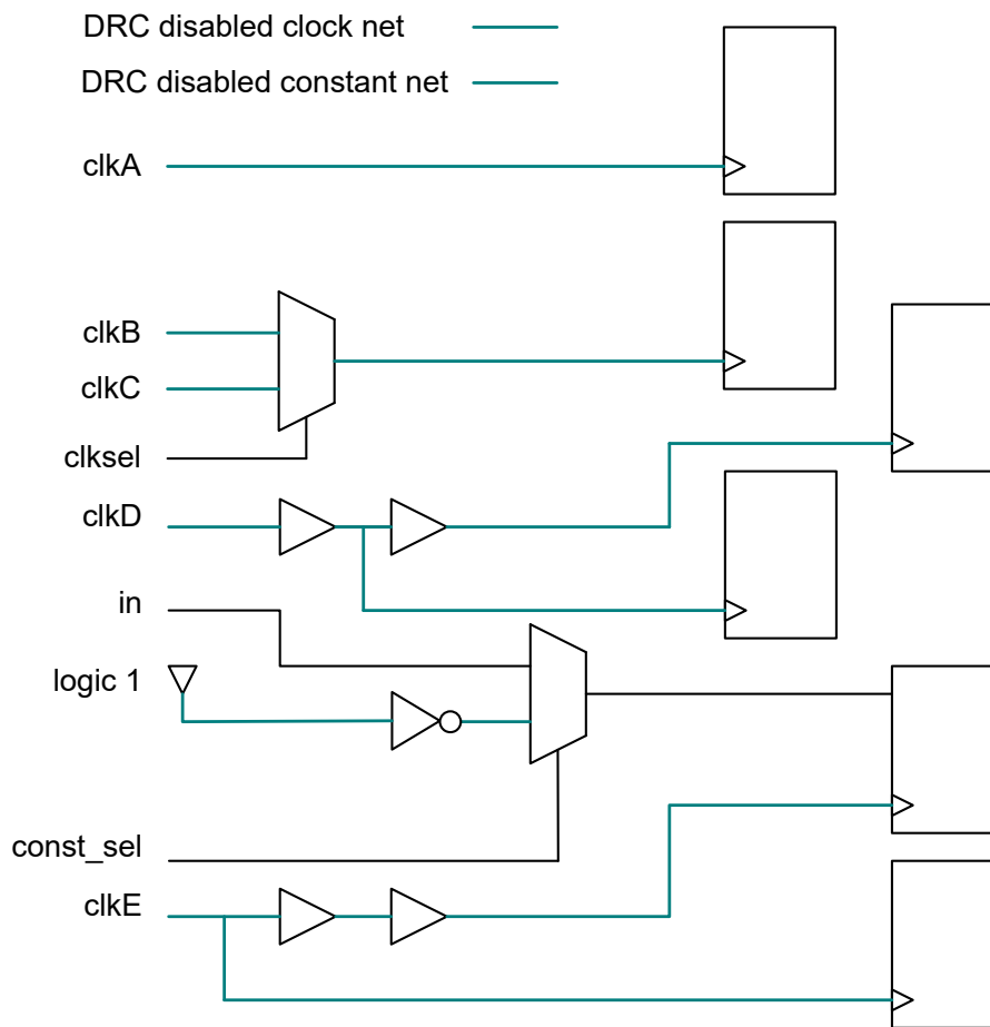
Figure 21 DRC Disabled Clock and Constant Nets Highlighted
