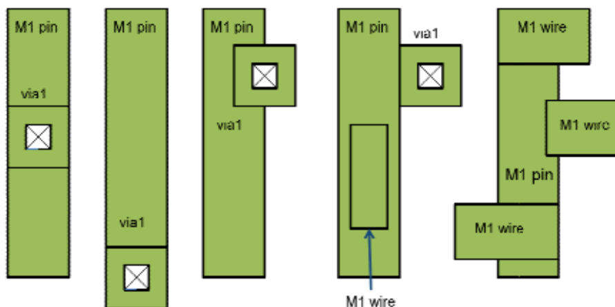
Figure 74 Unrestricted Pin Connections
