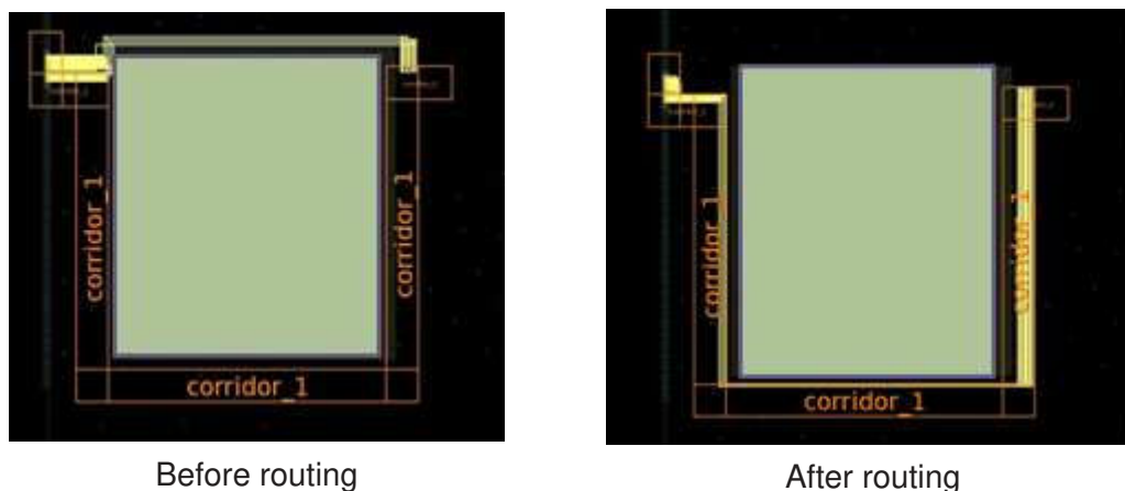
Figure 66 Using a Routing Corridor
