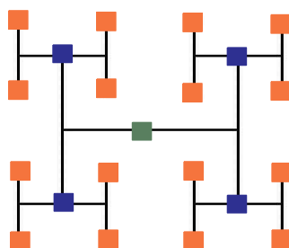
Figure 49 Clock Drivers Placed in an H-Tree Structure
