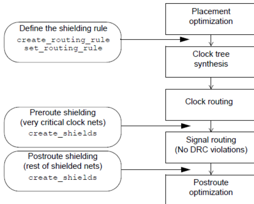
Figure 78 Zroute Shielding Flow
