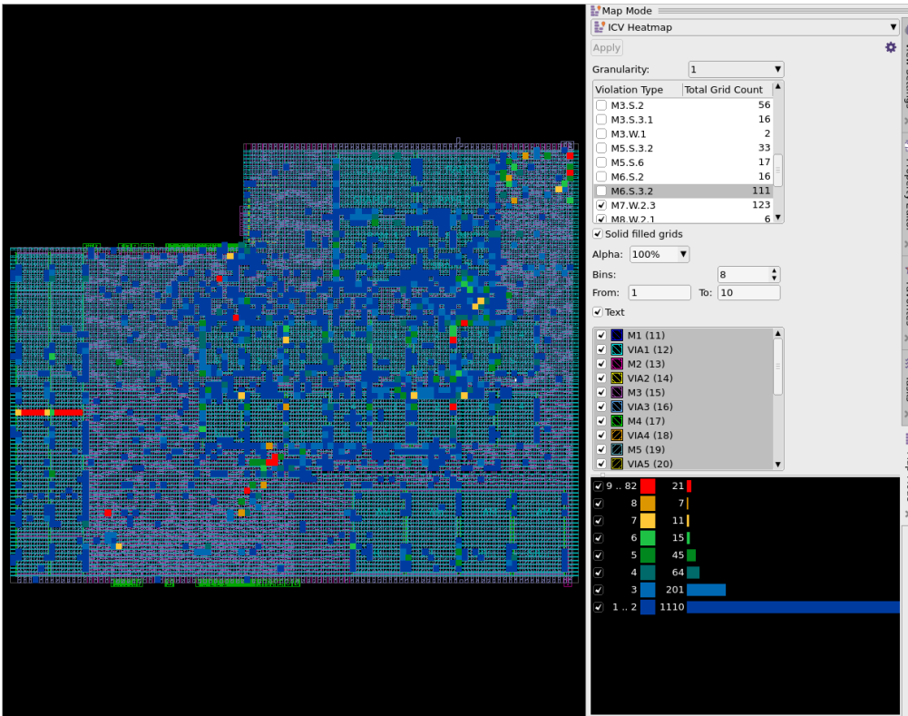
Figure 102 Bins Value Set to 8
