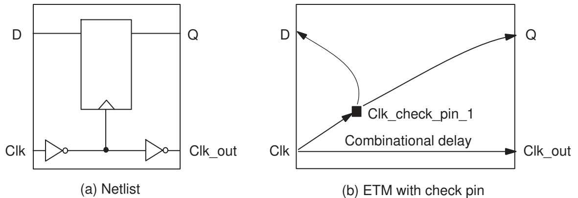
Figure 37 Module With Combinational Clock Path
