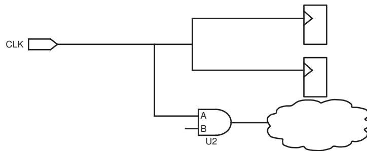
Figure 35 User-Defined Ignore Pin
