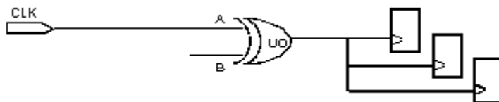
Figure 32 Non-Unate Gated Clock
