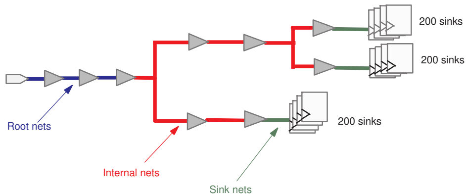
Figure 68 Root, Internal, and Sink Clock Net Types
