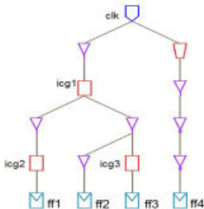
Figure 59 Segments and Subtrees of a Clock Tree
