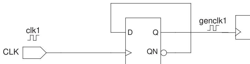
Figure 33 Nested Clock Tree With a Generated Clock
