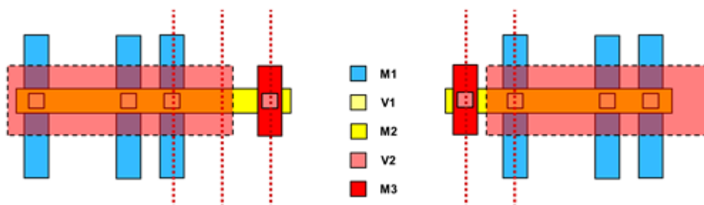
Figure 73 Pattern-Based Must-Join Pin Connection With Staggering
