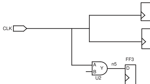
Figure 36 Specifying Exceptions on Pins Beyond the Clock Network
