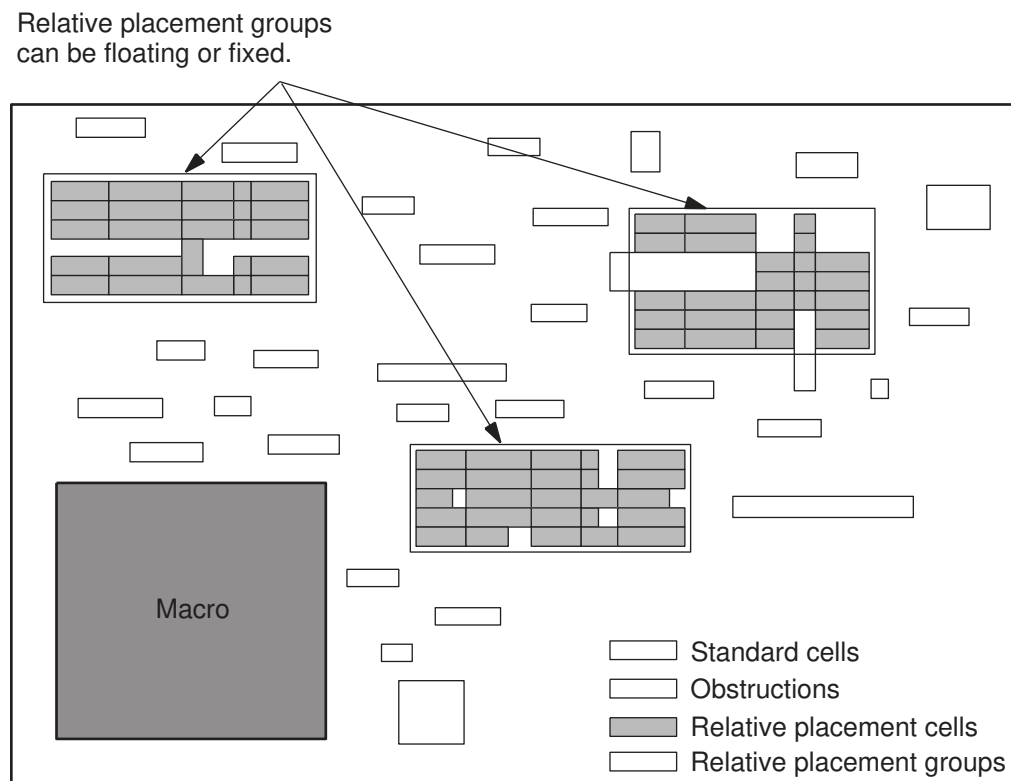
Figure 127 Relative Placement in a Floorplan
