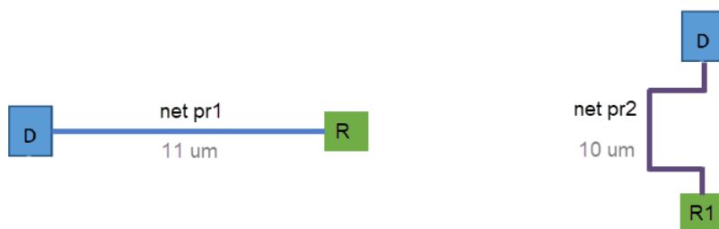
Figure 116 Minimum Wire Length Constraint for pr* Nets
