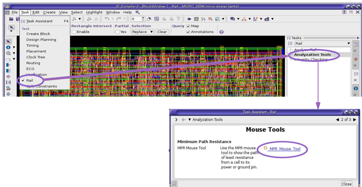
Figure 165 Invoking the MPR Mouse Tool
