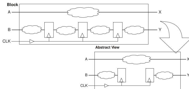
Figure 148 A Block and Its Abstract View
