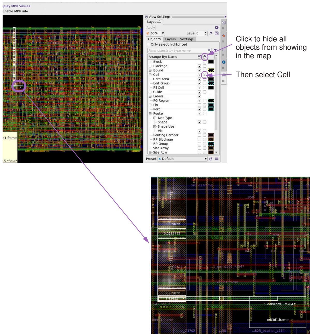
Figure 166 Tracing the Path With the Least Resistance
