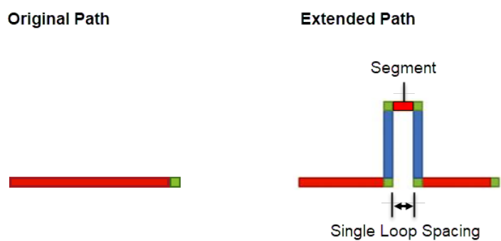
Figure 125 Adding Single Loops to Extend Wires
