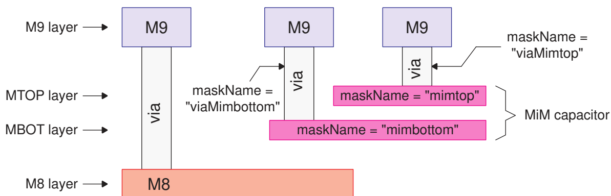
Figure 88 Cross-Section View of MiM Capacitor Layers
