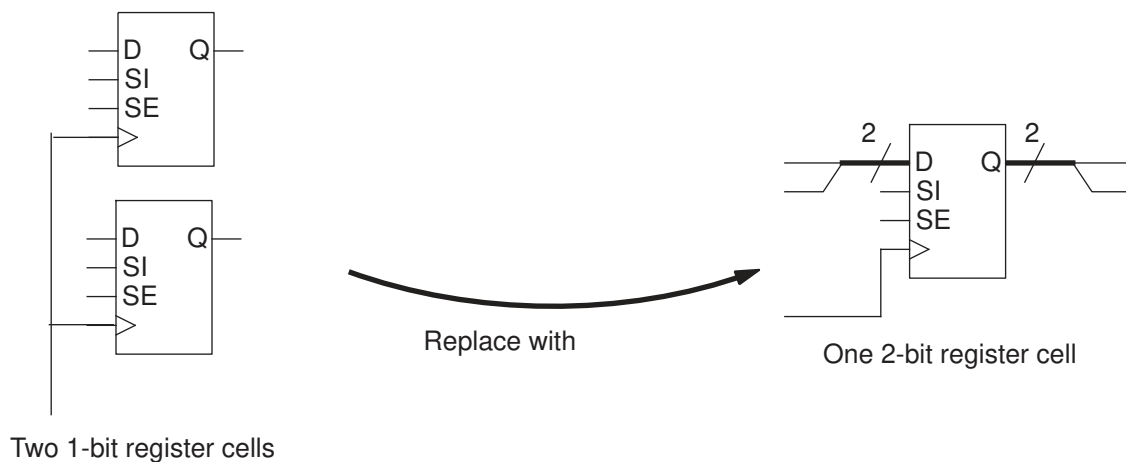
Figure 25 Replacing Multiple Single-Bit Register Cells With a Multibit Register Cell
