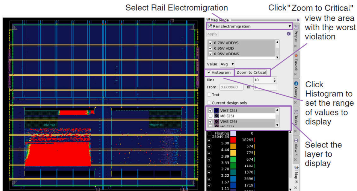
Figure 161 Displaying a PG Electromigration Map
